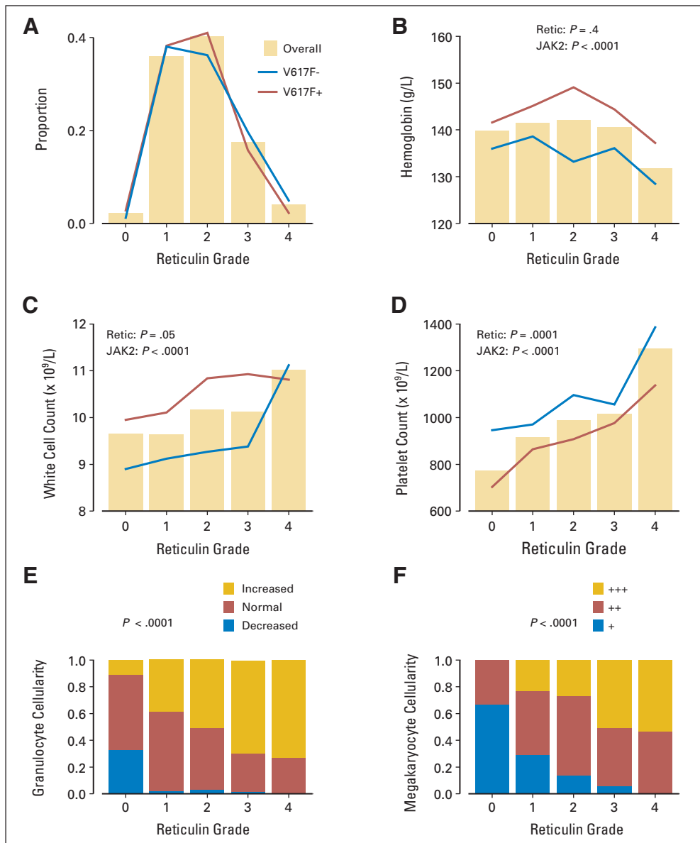
Fig 1. Association of reticulin grade at diagnosis with presentation laboratory features. (A) Histogram showing the frequency distribution of reticulin grades in the cohort of patients with essential thrombocythemia studied. The red and blue lines show the frequency distributions for JAK2 -positive and JAK2 -negative patients, respectively. (B) Mean hemoglobin levels across reticulin grades for the cohort as a whole (beige bars), as well as JAK2 -positive patients (red line) and JAK2 -negative patients (blue line) separately. (C) Mean white blood cell counts across reticulin grades for the cohort as a whole (beige bars), as well as JAK2 -positive patients (red line) and JAK2 -negative patients (blue line) separately. (D) Mean platelet counts across reticulin grades for the cohort as a whole (beige bars), as well as JAK2 -positive patients (red line) and JAK2 -negative patients (blue line) separately. (E) Distribution of bone marrow granulocyte cellularity by reticulin grade for the cohort. (F) Distribution of bone marrow megakaryocyte cellularity by reticulin grade for the cohort. Retic, reticulin; (+), mild increase; (++) moderate increase; (+++), severe increase.
